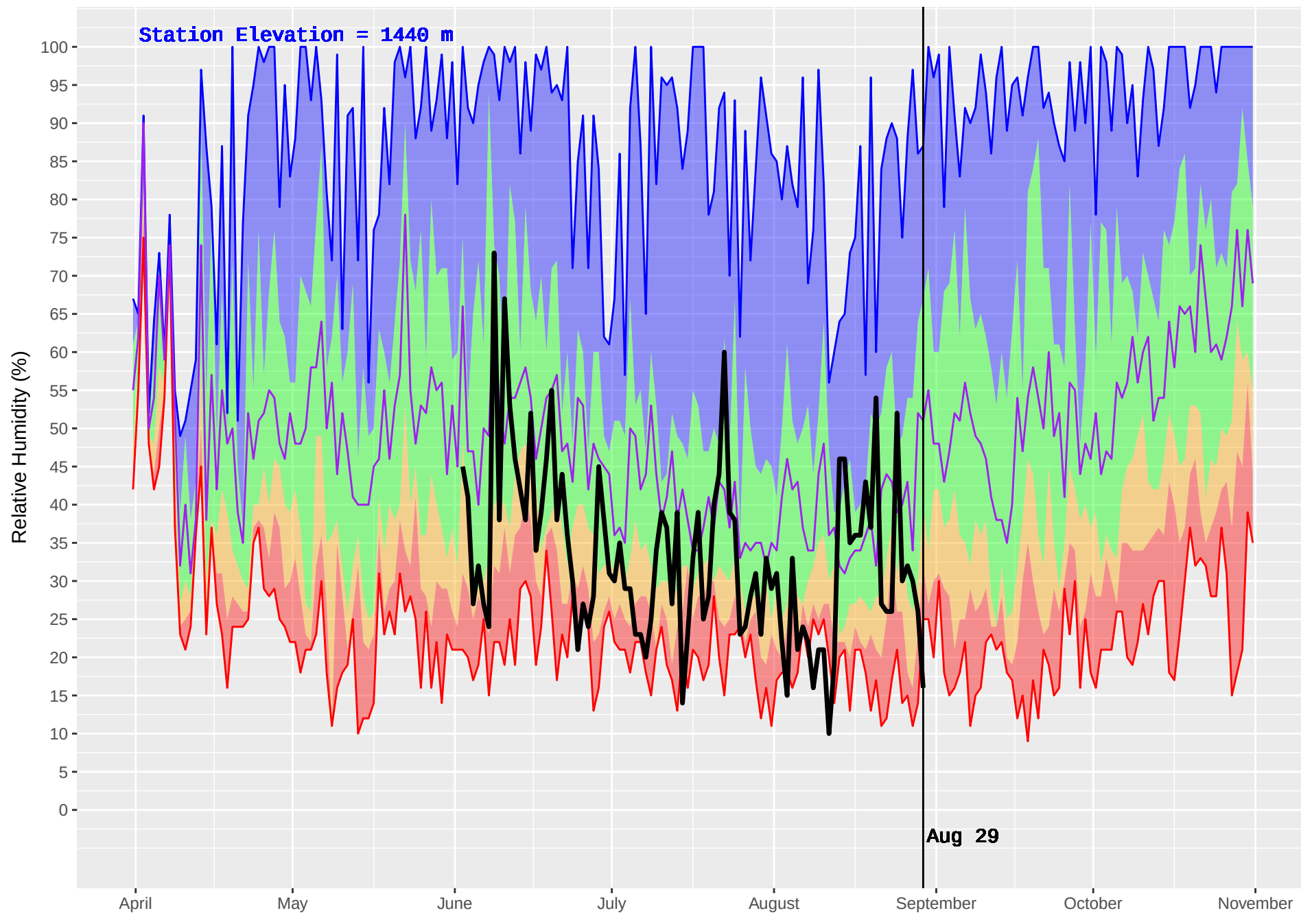
PASKA LAKE (326) : Historical (1999–2016) and Current (2017) Noon Relative Humidity
