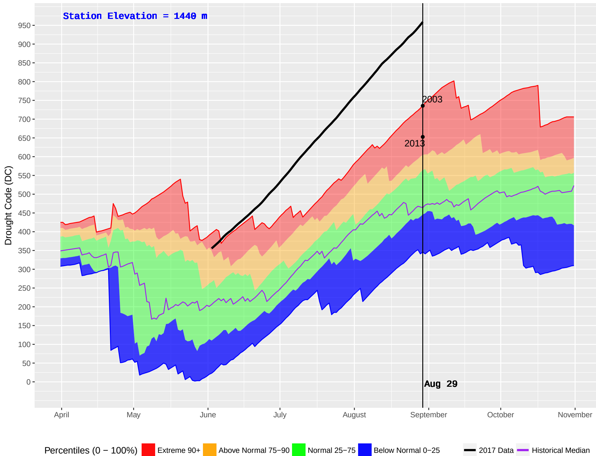
PASKA LAKE (326) : Historical (1999–2016) and Current (2017) Noon Drought Code (DC)
