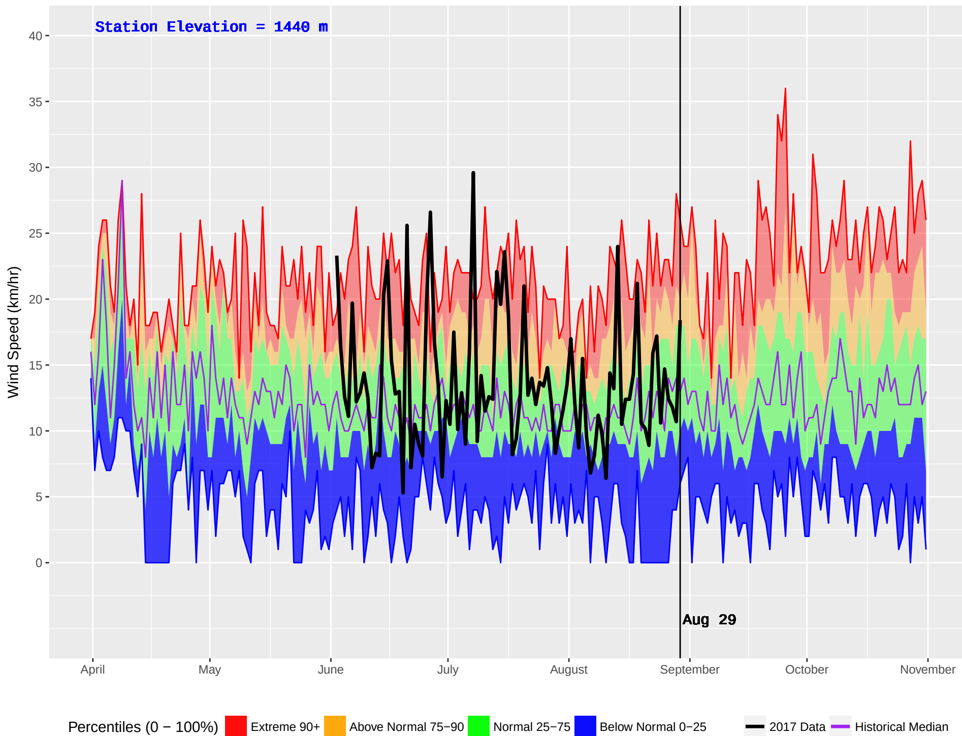
PASKA LAKE (326) : Historical (1999–2016) and Current (2017) Noon Wind Speed
