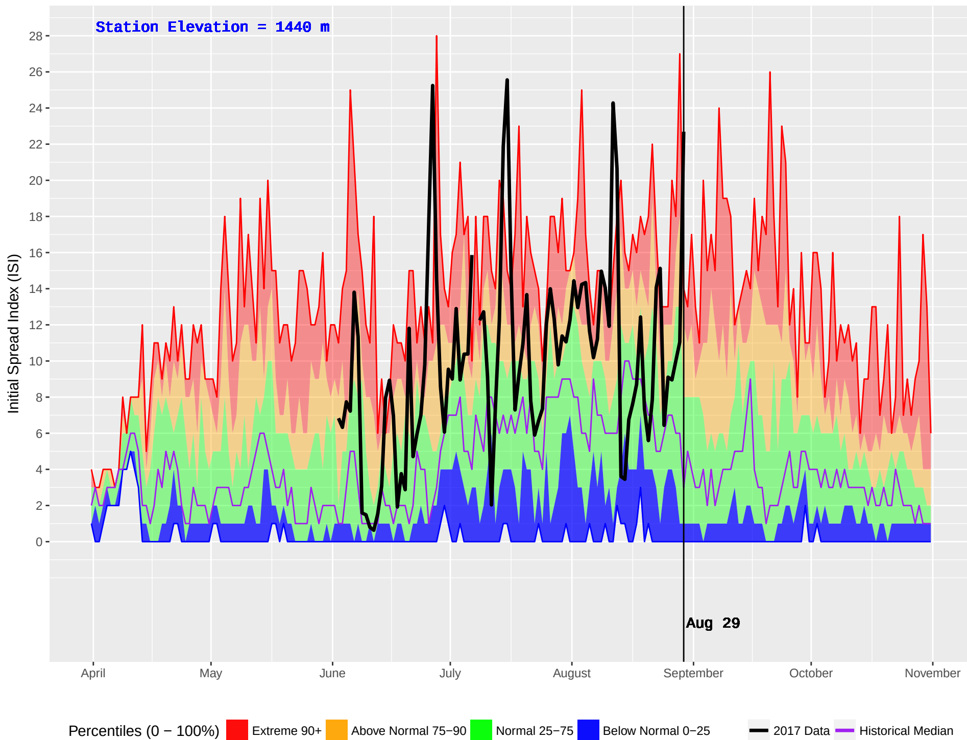
PASKA LAKE (326) : Historical (1999–2016) and Current (2017) Noon Initial Spread Index (ISI)
