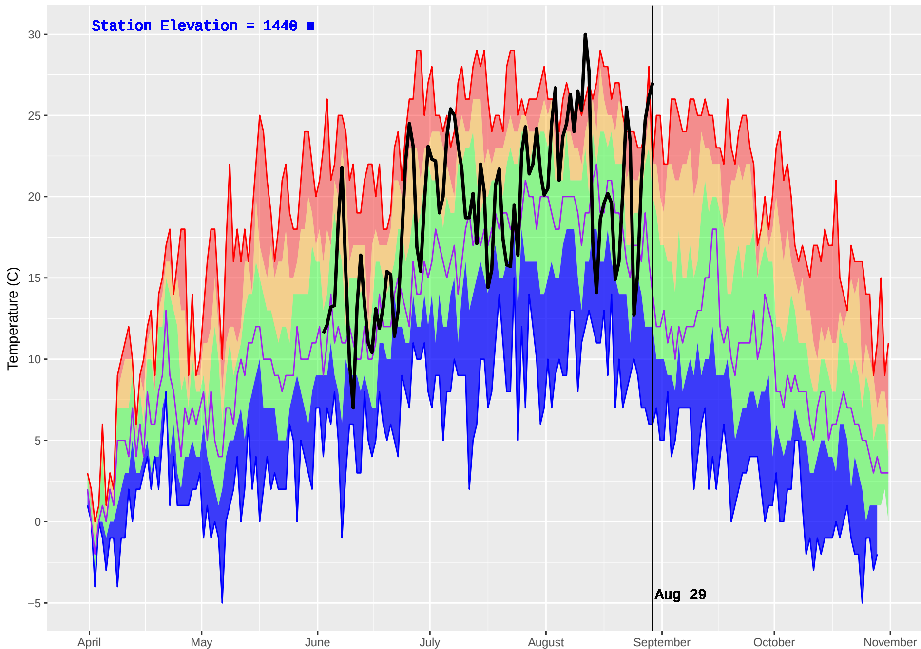
PASKA LAKE (326) : Historical (1999–2016) and Current (2017) Noon Temperature
