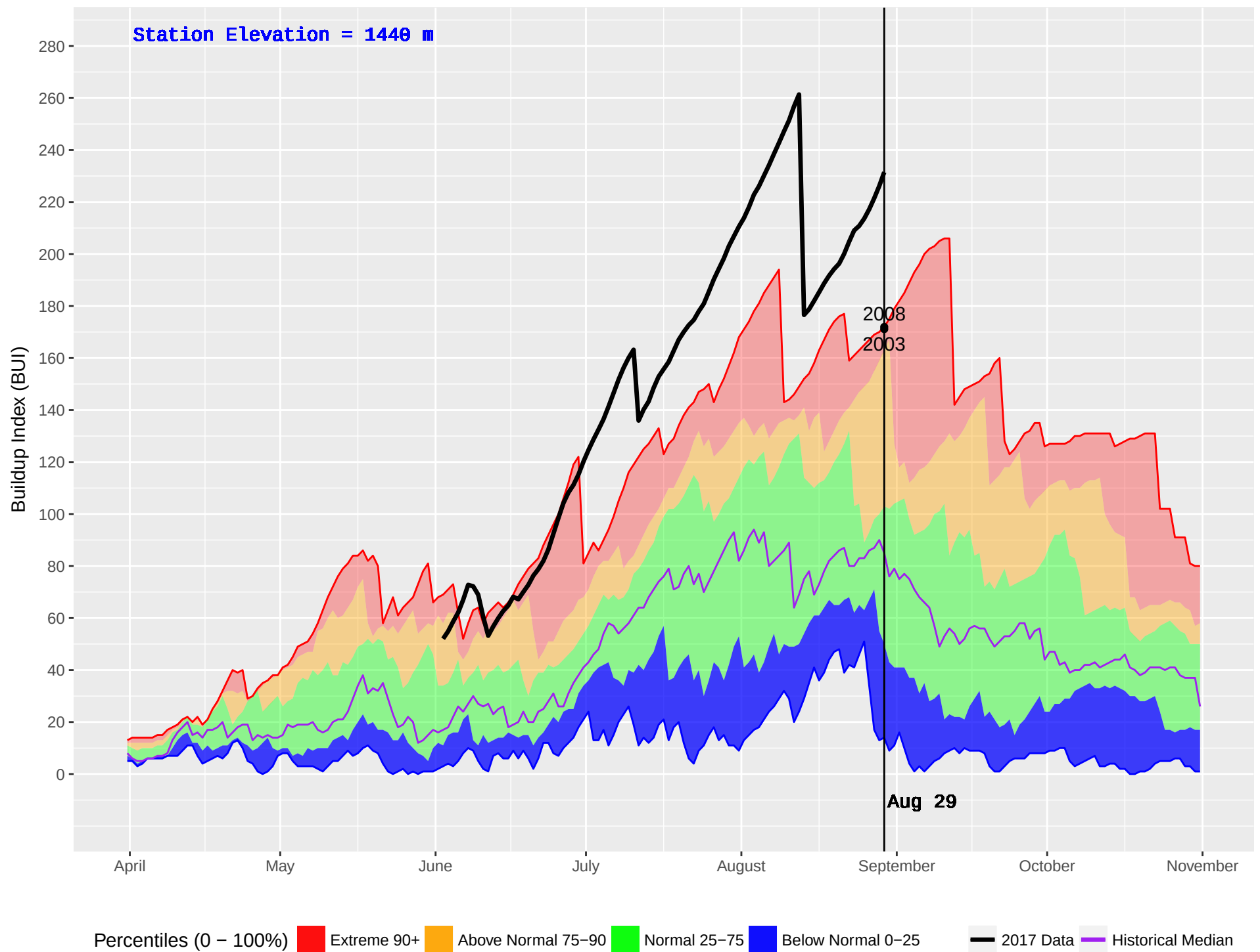
PASKA LAKE (326) : Historical (1999–2016) and Current (2017) Noon Buildup Index (BUI)
