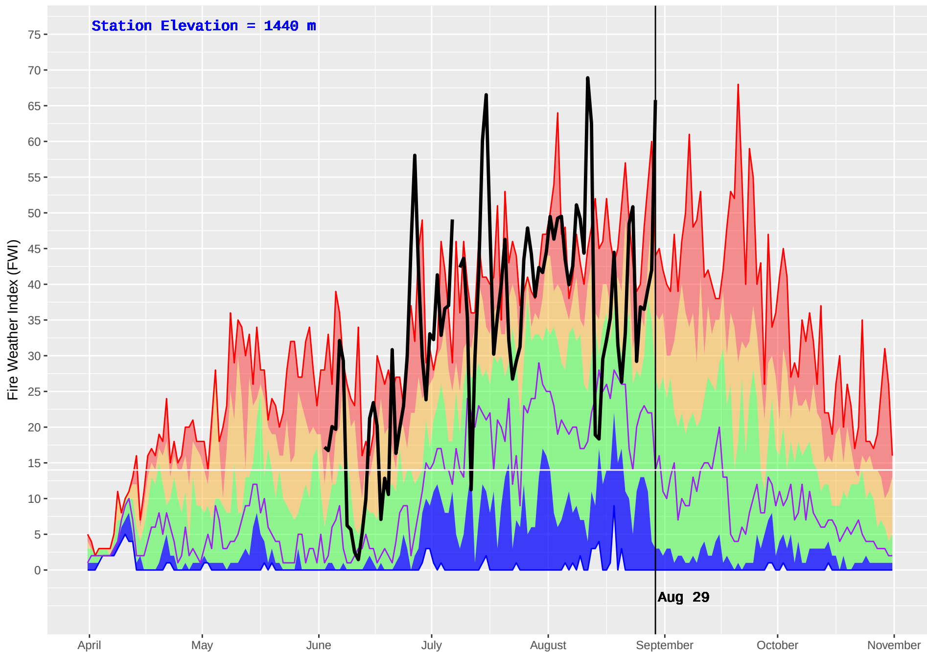
PASKA LAKE (326) : Historical (1999–2016) and Current (2017) Noon Fire Weather Index (FWI)
